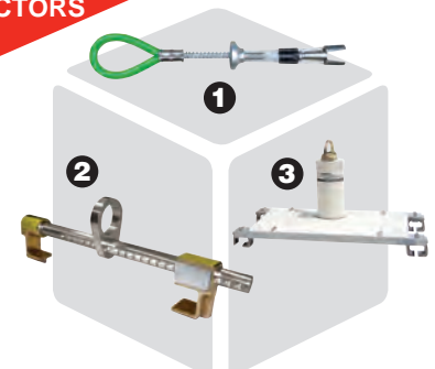
1. Miller Grip Anchor 2. Miller ShadowLite Beam Anchor 3. Miller Fusion Roof Anchor Post
